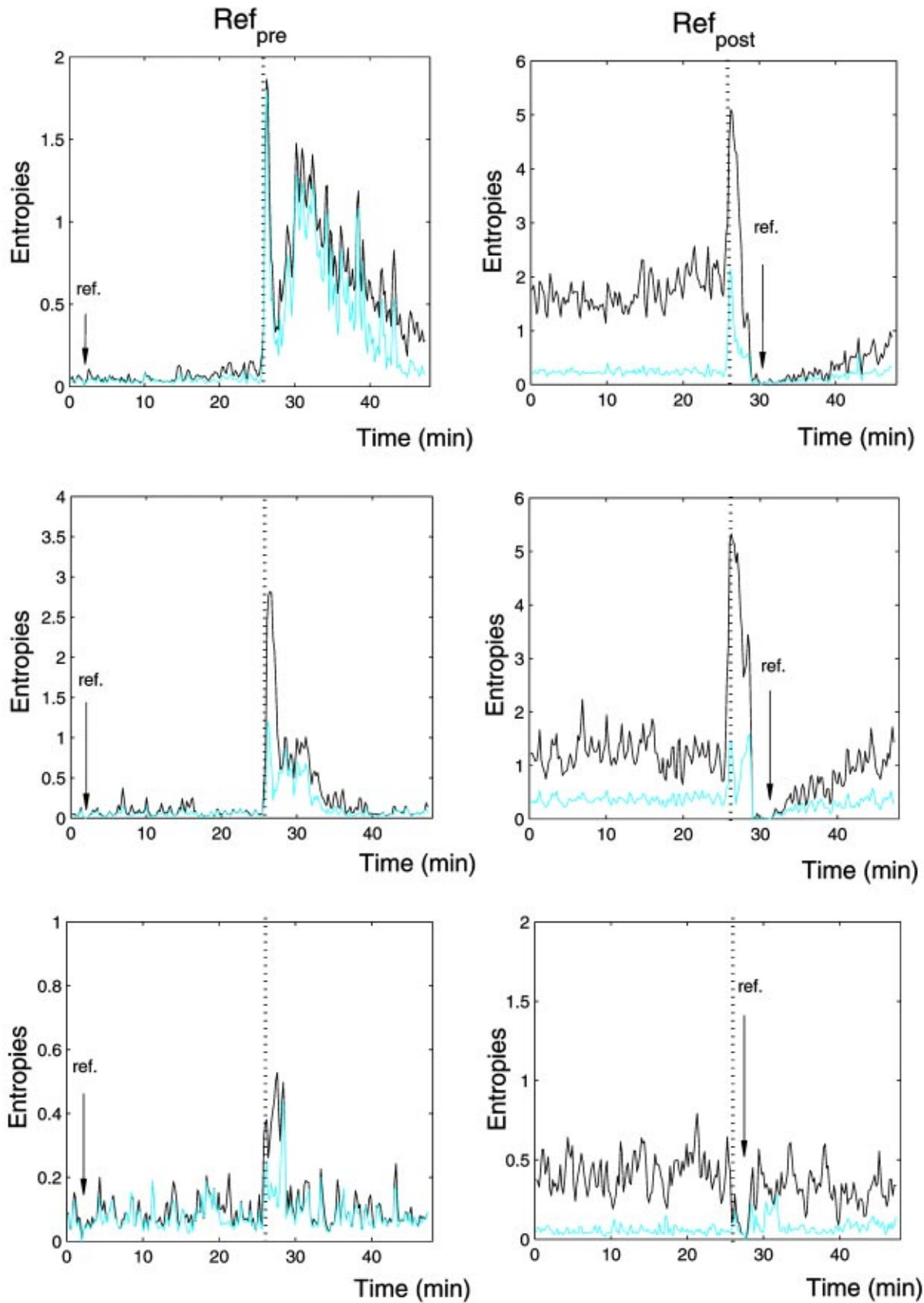
FIG. 1. Kullback-Leibler (black line) and renormalized (gray line) entropies from EEGs recorded in the seizure-generating area (upper row), adjacent to the seizure generating areas (middle row), and in the nonaffected brain hemisphere (lower row). Data shown in left (right) columns were obtained from using a pre-(post-) seizure reference window (marked by an arrow). The dotted vertical lines mark the electrical onset of the seizure.
